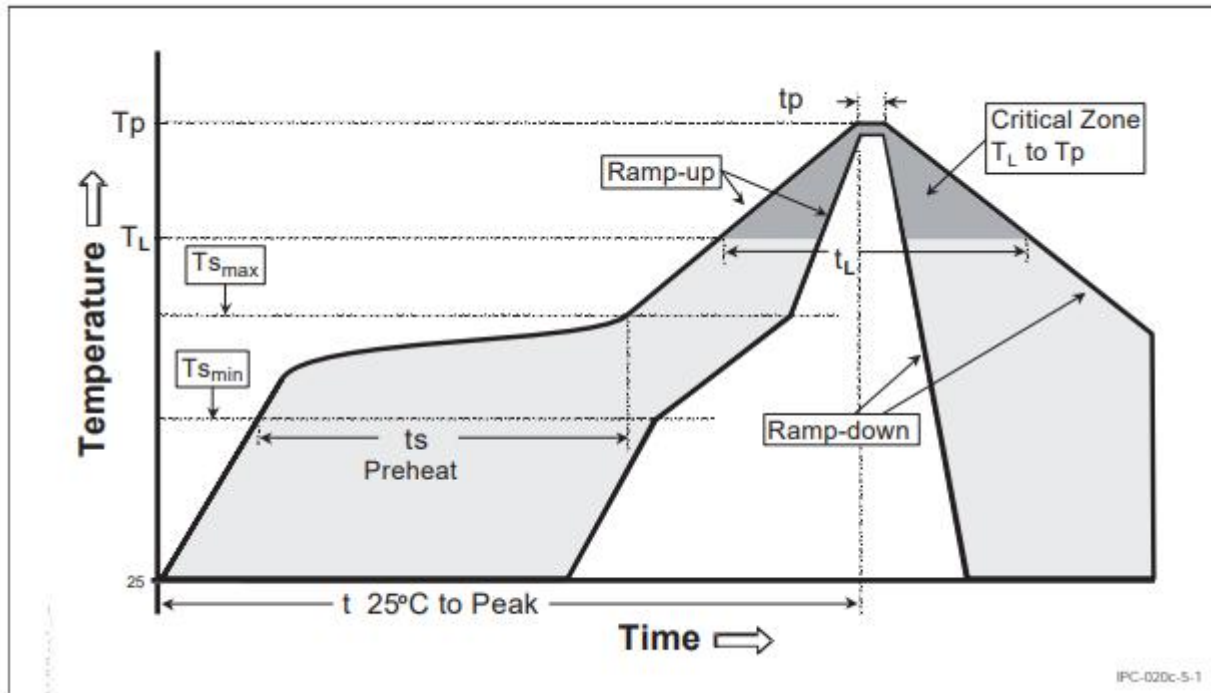
Figure 17 Reflow curve
