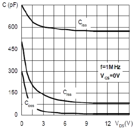
Figure 7 Capacitance
