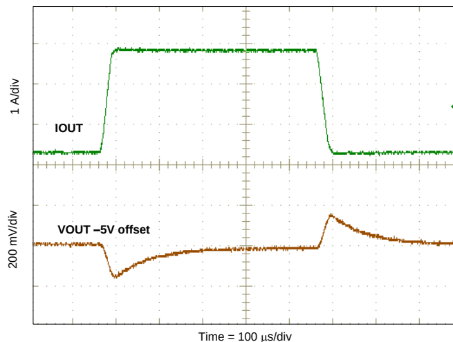
Figure 36. Load Transient
