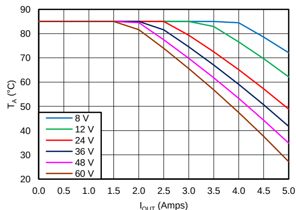
Figure 57. 5V Outputs
