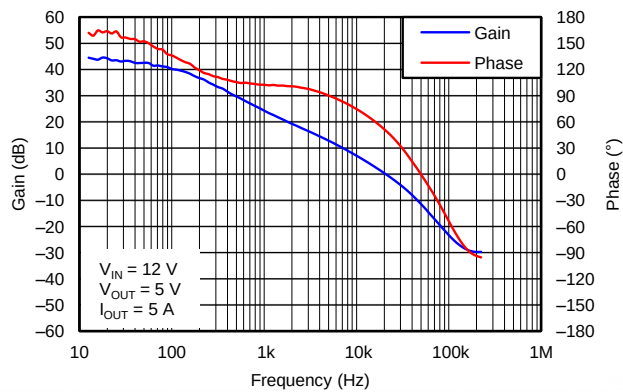
Figure 53. Overall Loop Frequency Response
