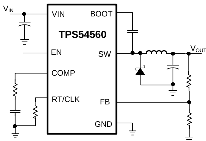
SIMPLIFIED SCHEMATIC
