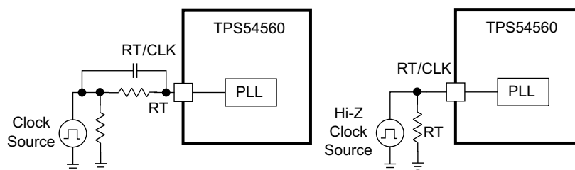
Figure 27. Synchronizing to a System Clock
